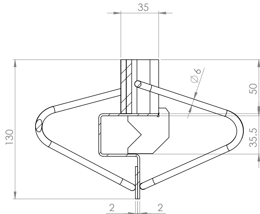
SECTION C-C SCALE 1 : 2
